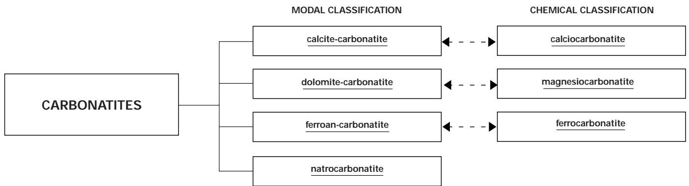
Figure 25 Hierarchical classification of carbonatites.
