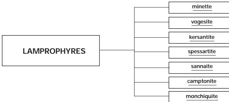
Figure 31 Hierarchical classification of lamprophyres.
