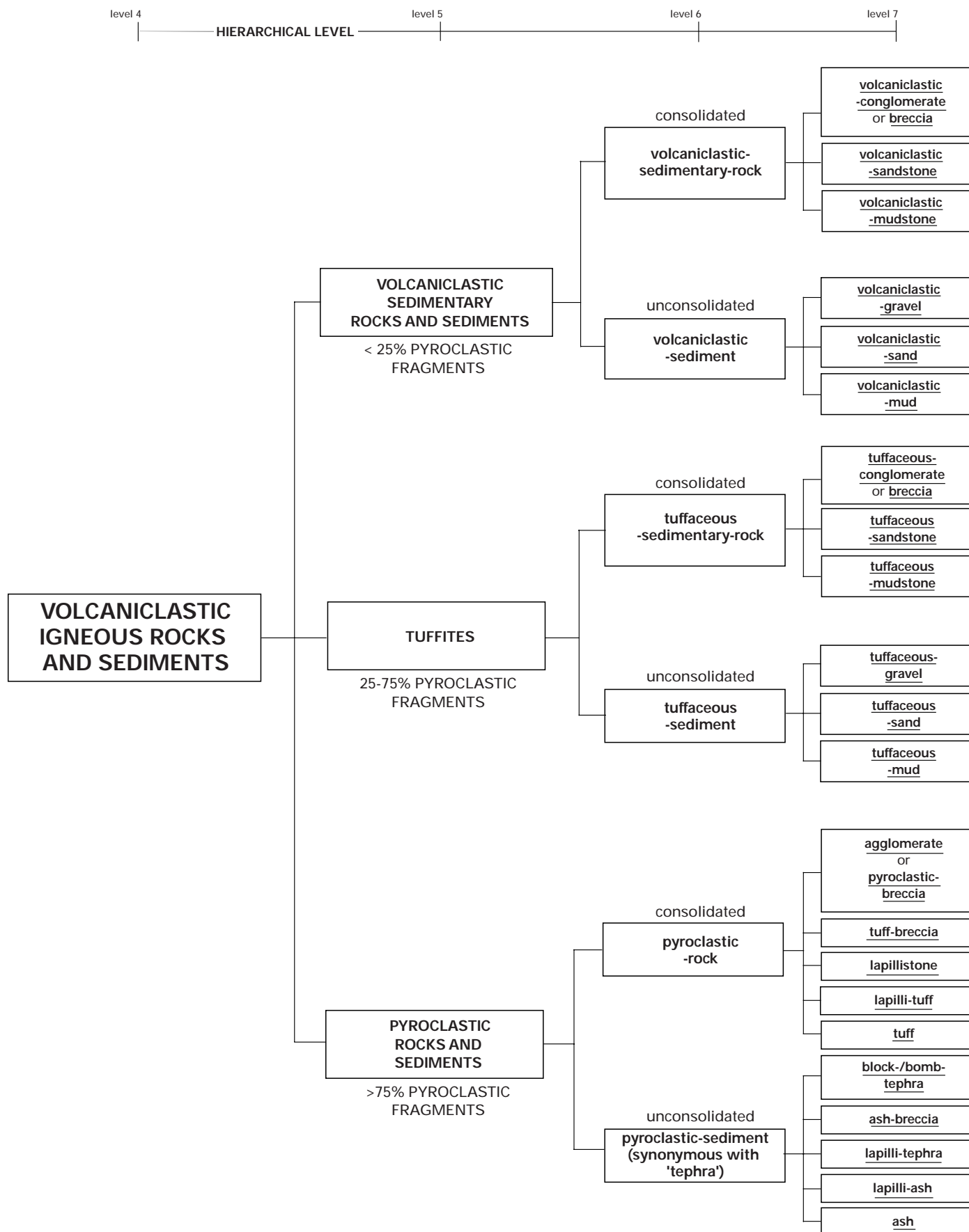
Figure 4 Hierarchical classification of volcanoclastic igneous rocks and sediments.
