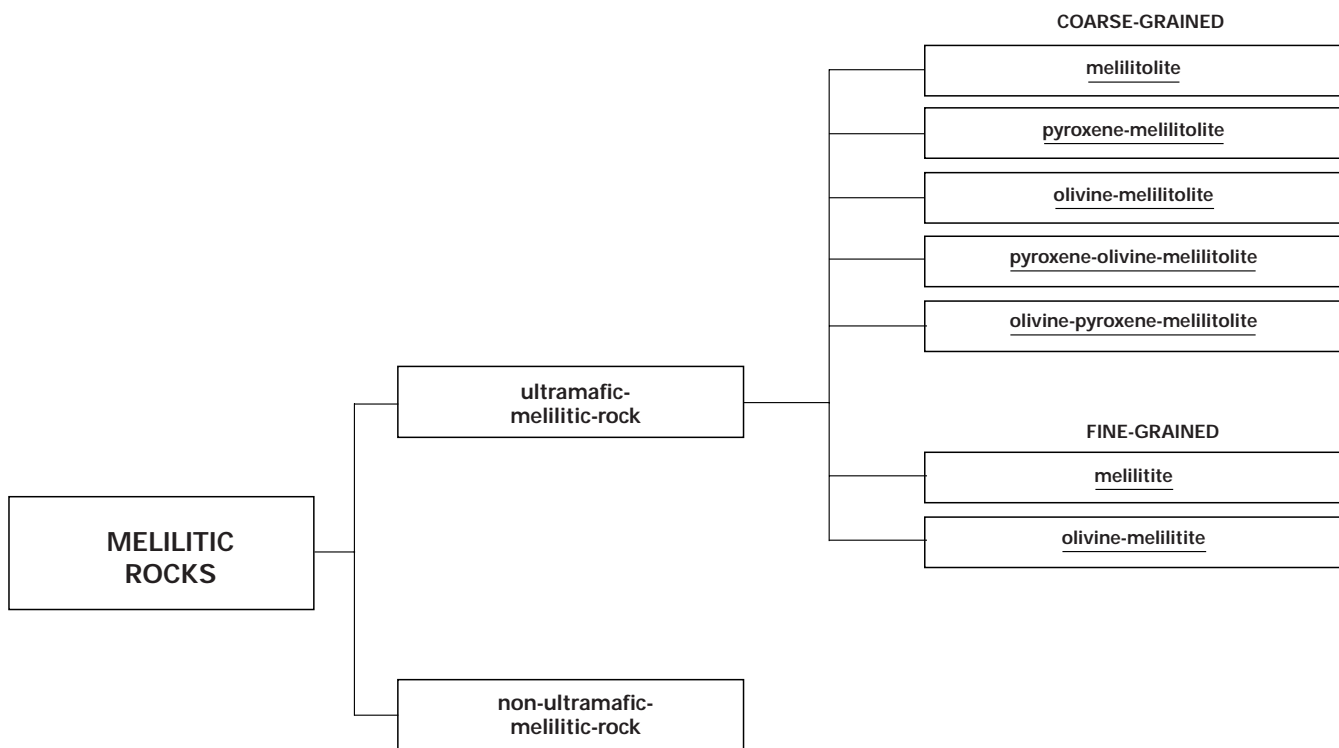
Figure 27 Hierarchical classification of melilitic rocks.
