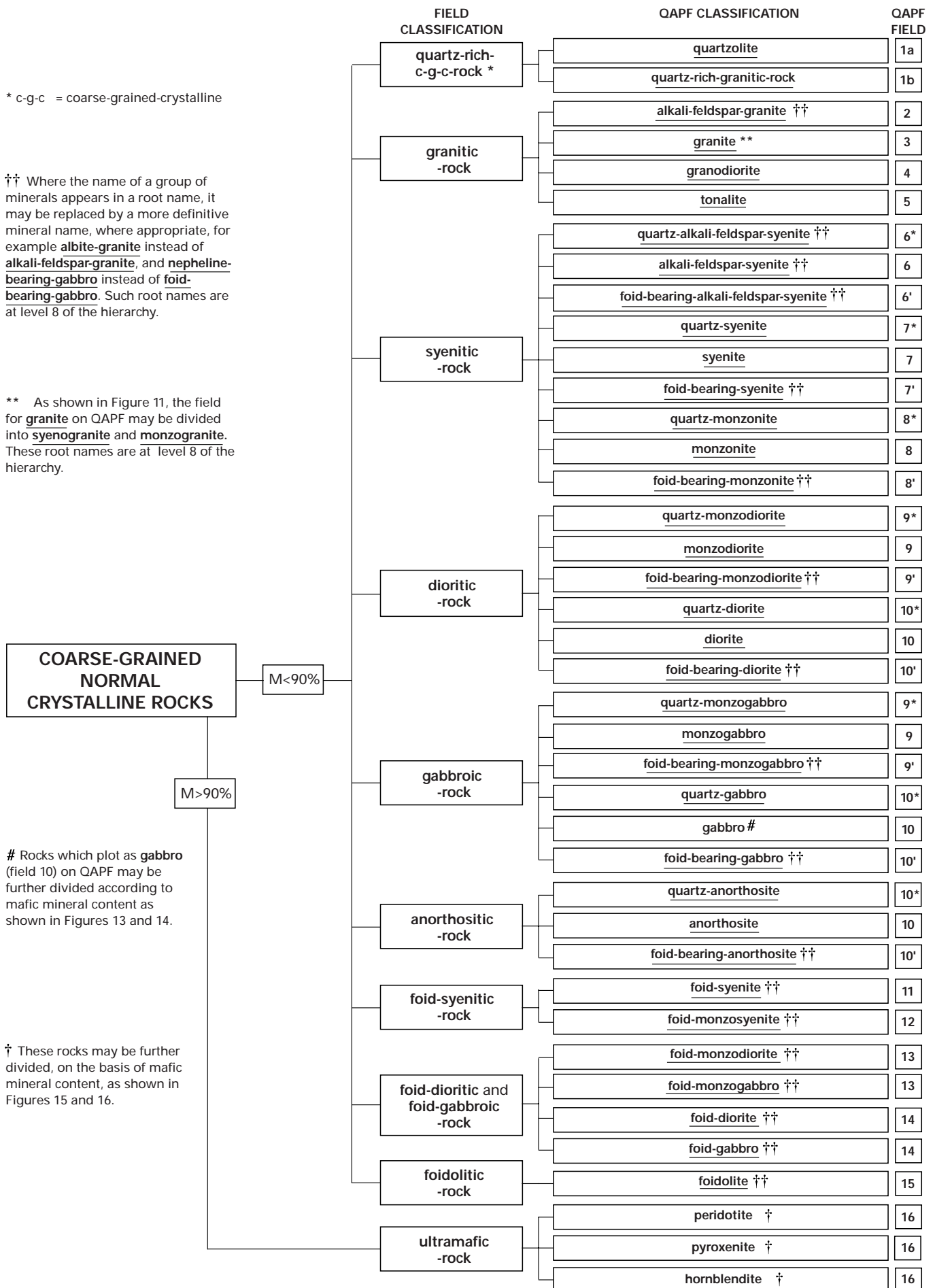
Figure 9 Hierarchical classification of coarse-grained normal crystalline rocks.
